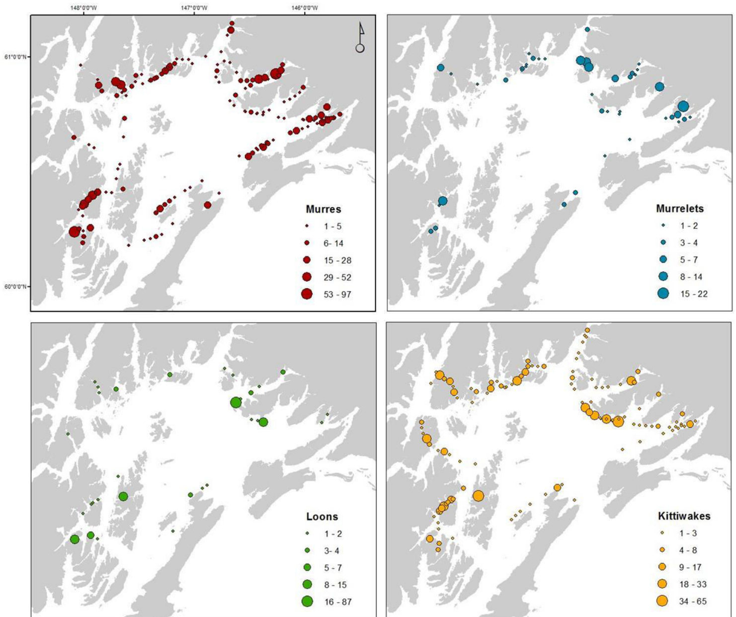
Figure 7. Distribution of common murre, Brachyramphus murrelets (Kittlitz's and marbled murrelets), loons (common loon, Pacific loon, red-necked loon, and yellow-billed loon) and black-legged kittiwakes recorded during October & November 2015 surveys ( n = 2 ) in Prince William Sound. Note that scales for each figure legend vary by species.
