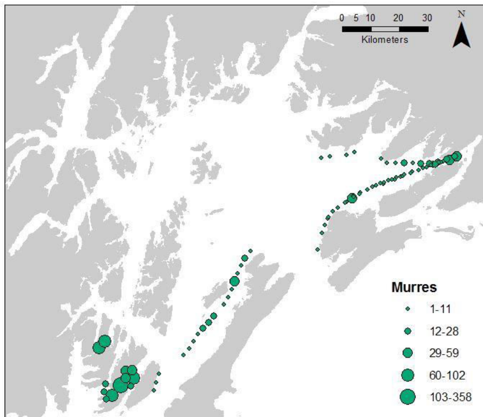
Figure 2: The highest densities of common murren to date were observed in the southwest passages of Prince William Sound during February 2015, immediately prior to the die-off beginning in March 2015.
